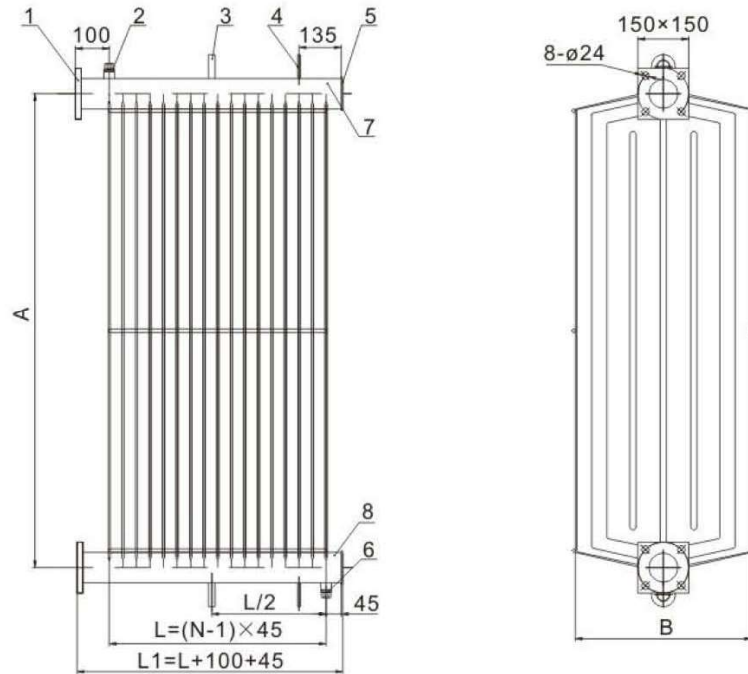
PC、PG型外焊式散热片 (图1) PC and PG type outer-welding fins (Fig. 1)
